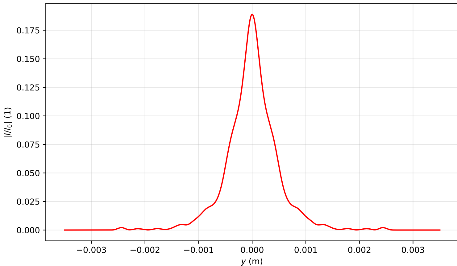
Intensity profile I(x=0, y, z=3.025)/I_0 , \text{Pin}=5.0\text{Pcr} , artificial time
